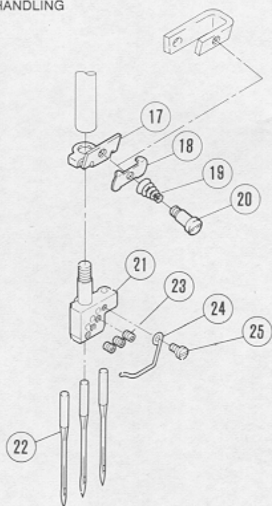
針糸・飾り糸機構 NEEDLE-SPREADER THREAD HANDLING
